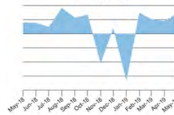
Volatility (13 mo)
