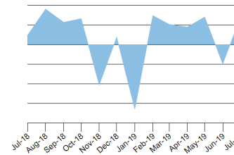
Volatility (13 mo)
