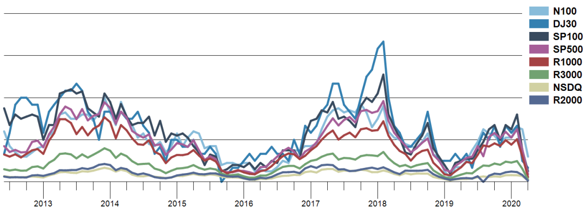
Mapper Score™ for S&P 500 Stocks Mapped = 23 Mapper Score = 4.60%
