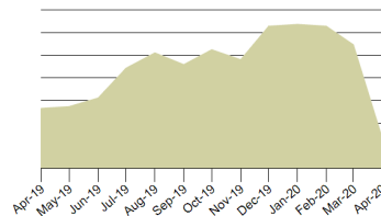
Mapper Score™ for NASDAQ Stocks Mapped = 23 Mapper Score = 0.85%
