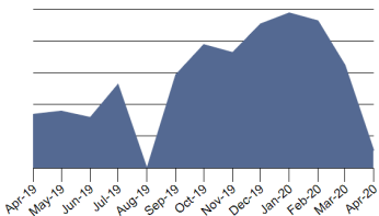
Mapper Score™ for Russell 2000 Stocks Mapped = 10 Mapper Score = 0.50%
