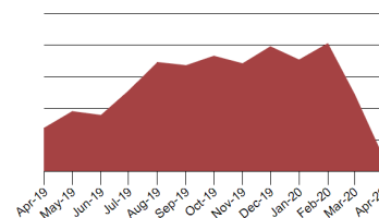
Mapper Score™ for Russell 3000 Stocks Mapped = 43 Mapper Score = 1.43%
